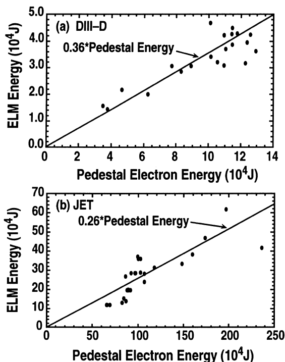
Fig. 1. The ELM energy loss, \Delta W , versus the pedestal electron pressure integrated over the plasma volume for: (a) DIII-D; (b) JET.
