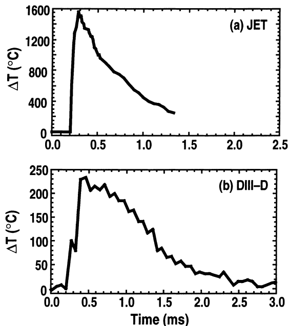
Fig. 3. The temperature rise of the divertor surface as a function of time for: (a) JET; (b) DIII-D. Time t=0 is the beginning of the data record. The temperature rise is coincident with onset of the ELM instability, within measurement uncertainty. Most of the temperature rise due to an ELM occurs in about 100 \mu s for JET and within 300 \mu s for DIII-D.
