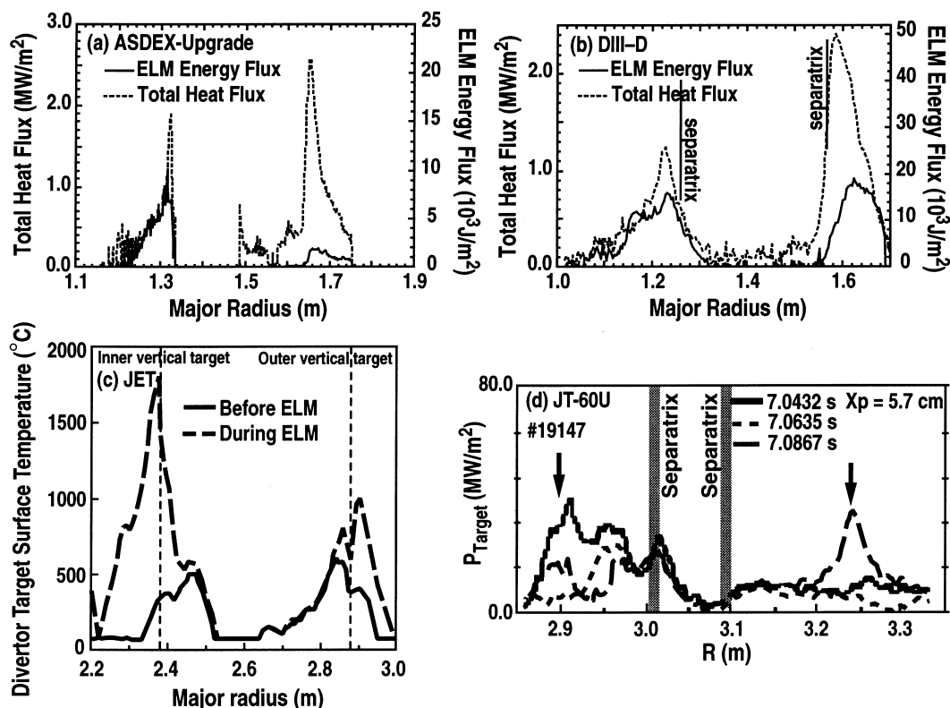
Fig. 2. ELM deposition profile for: (a) ASDEX-Upgrade; (b) DIII-D; (c) JET; (d) JT-60U. For ASDEX-Upgrade and DIII-D the total heat flux profile averaged over ELMs is also shown. The JET profile shows the surface temperature between and during ELMs. The three ELM profiles shown for JT-60U illustrate the variability of the profile for individual ELMs.
